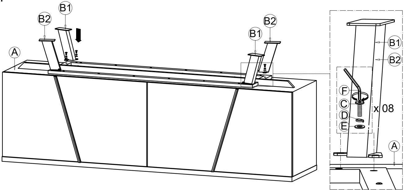
B2: Right Leg x 2
